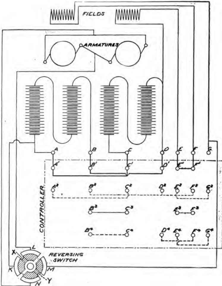
FIG. 303.—Diagram Plan of the Several Parts of an Electrical Vehicle Driving Circuit. The field-windings and armatures are shown projected, the proper wiring connections being indicated. The periphery of the controller is laid out within the broken line rectangle, the contacts and connections through it for varying the circuits through four speeds being shown. A, B, C, D, E, F, G are the terminal contact points of the various speed circuits, to be made as the positions of the controller contacts are varied. A', B', C', D', E', F' are the controller contacts, which, with those already mentioned, make the proper circuits for the first speed. Similarly, A², B², C², etc., when brought into contact with A, B, C, etc., give the second speed circuits; B³, C³, E³, F³, in contact with A, B, C, D, etc., give the third speed; and B⁴, C⁴, D⁴, in the same manner, the fourth speed. The reverse switch gives the backward movement, as described.
